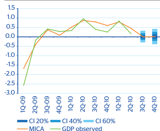
Chart 14 Eurozone: GDP growth and MICA model forecast (% q/q)
