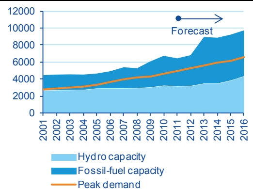
Chart 2 Effective capacity and peak demand (MW)
